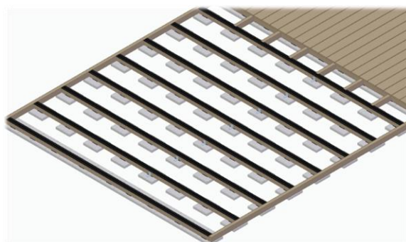
Joist tape used between decking and joists.
