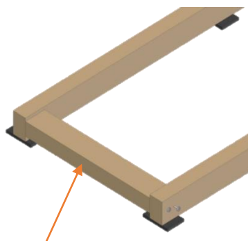
TIP: Fit the crossbeams horizontally to ensure good ventilation and drainage.
